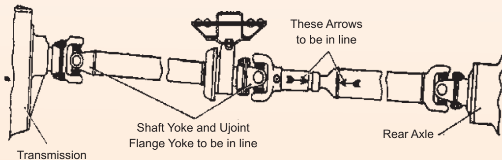
Fig: Arrangement of a Two-Piece Propeller Shaft
